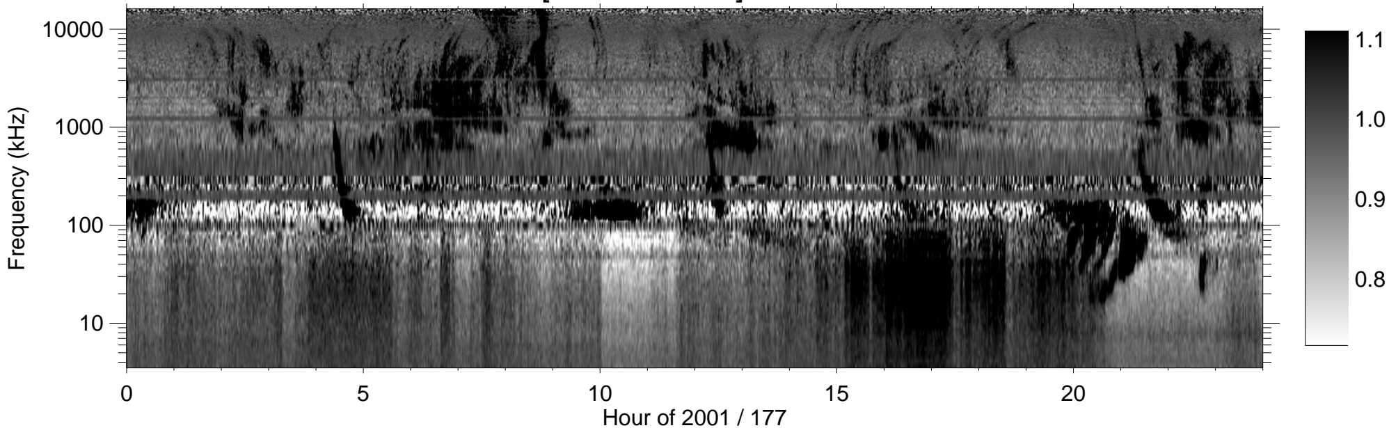
RPWS [ABCH1H2/Ex] (-B) 2001/06/26
