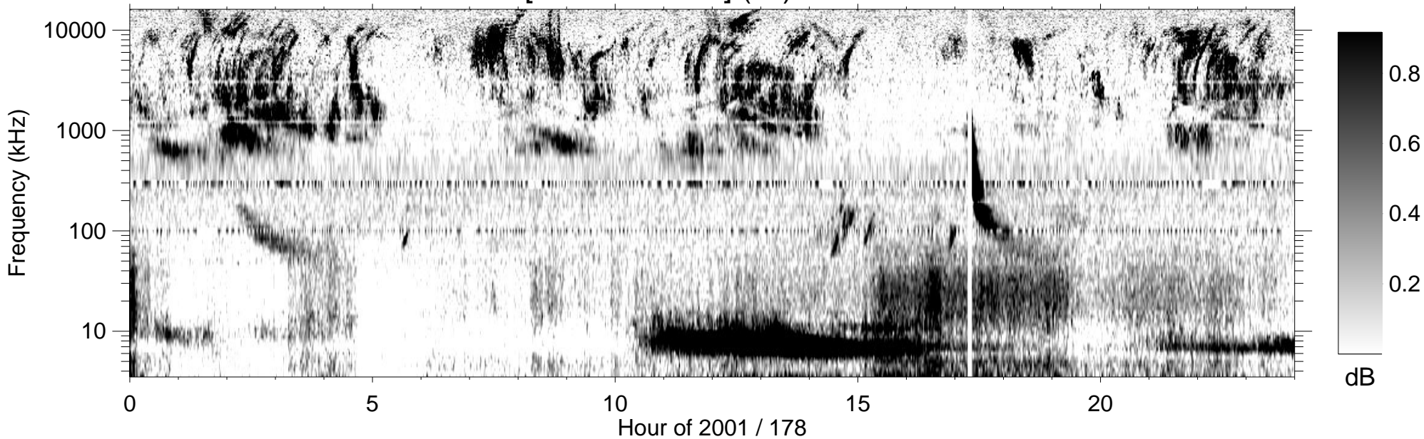
RPWS [ABCH1H2/Ex] (-B) 2001/06/27
