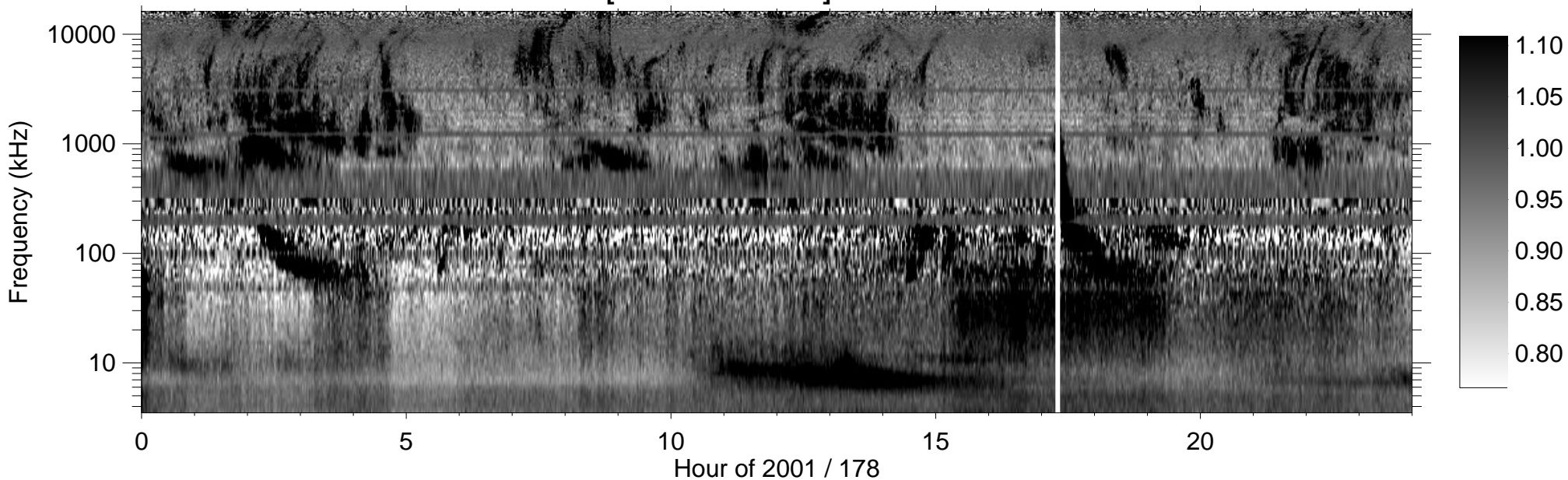
RPWS [ABCH1H2/Ex] (-B) 2001/06/27
