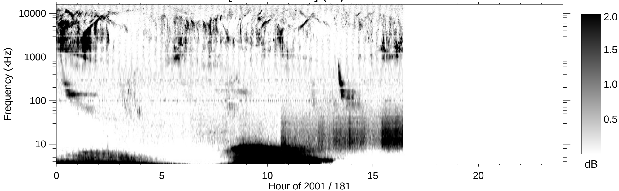
RPWS [ABCH1H2/Ex] (-B) 2001/06/30
