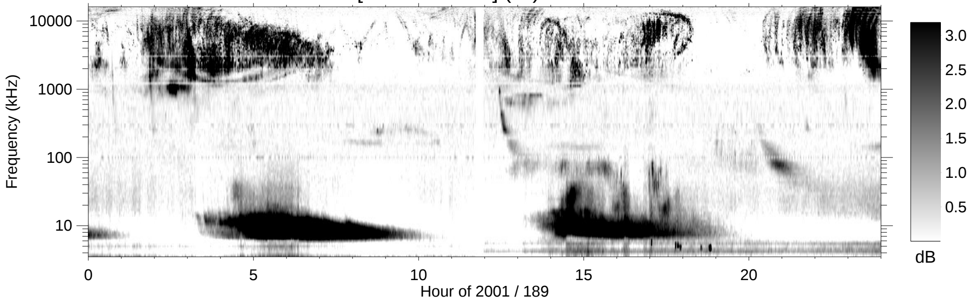
RPWS [ABCH1H2/Ex] (-B) 2001/07/08
