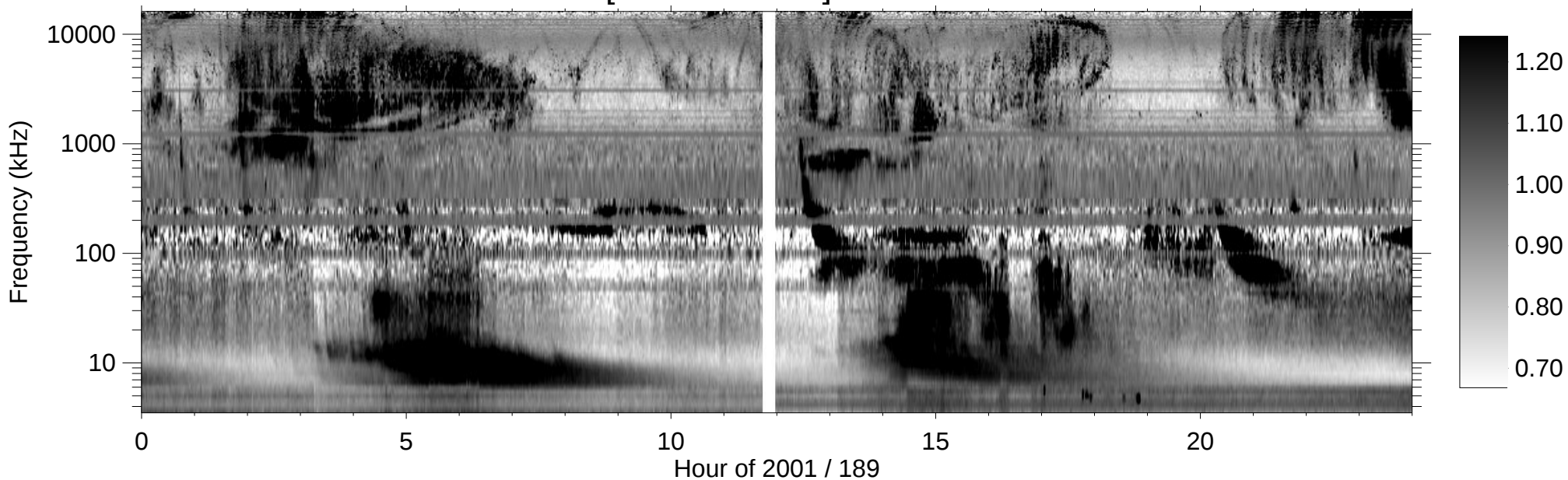
RPWS [ABCH1H2/Ex] (-B) 2001/07/08
