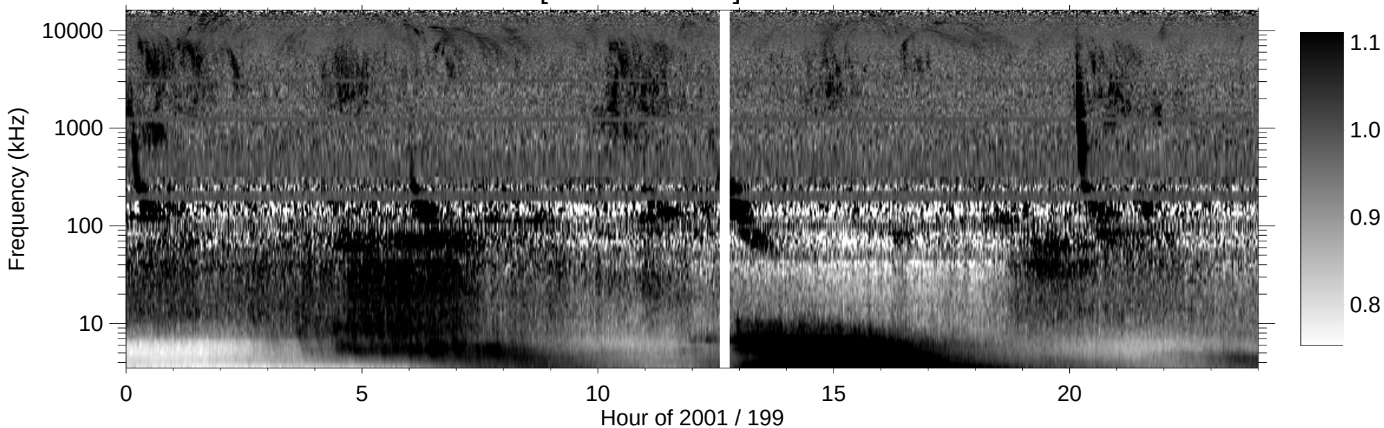
RPWS [ABCH1H2/Ex] (-B) 2001/07/18
