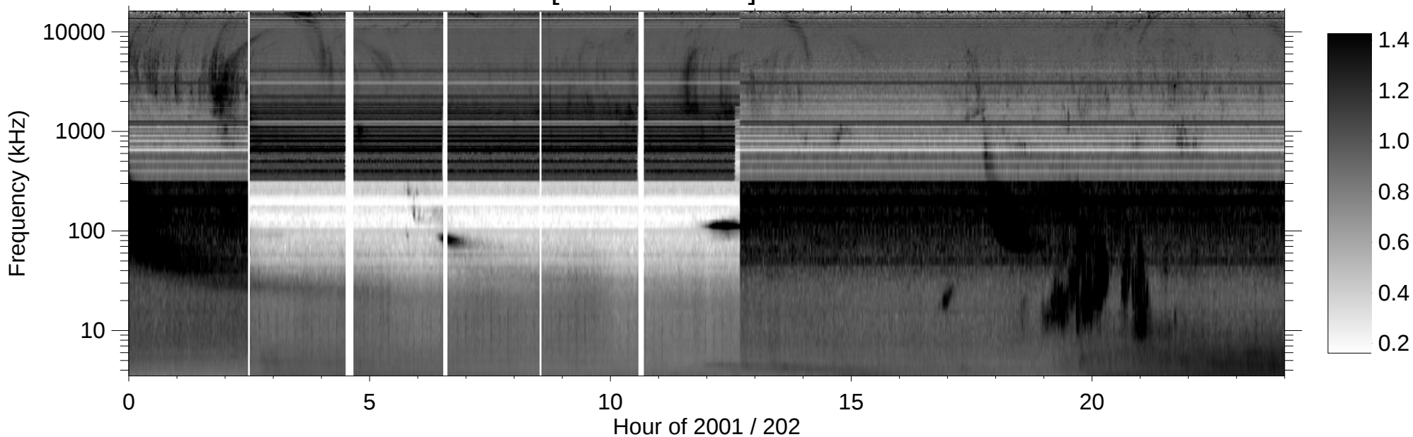
RPWS [ABCH1H2/Ex] (-B) 2001/07/21
