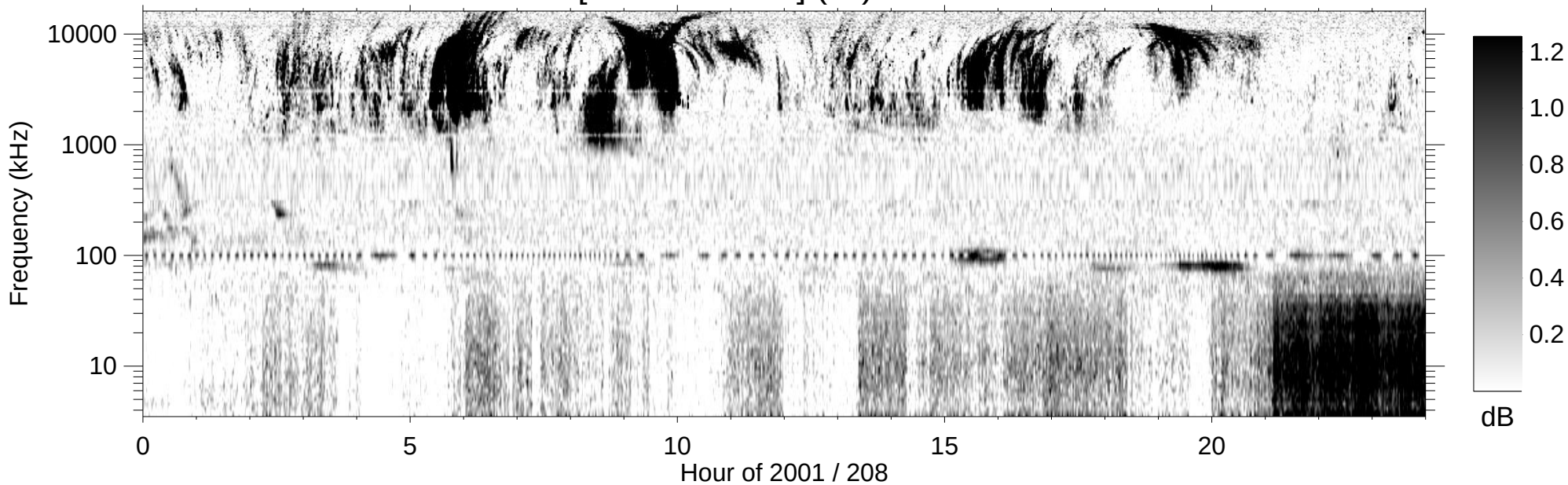
RPWS [ABCH1H2/Ex] (-B) 2001/07/27
