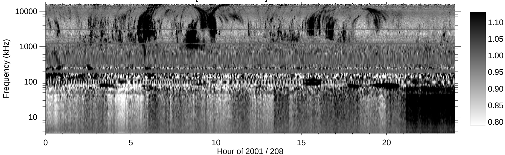
RPWS [ABCH1H2/Ex] (-B) 2001/07/27
