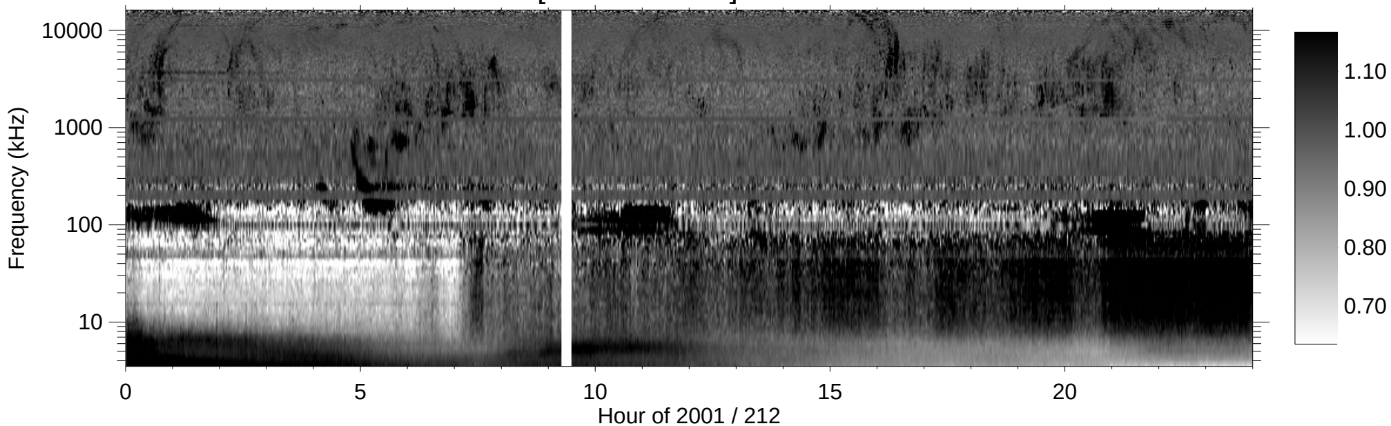
RPWS [ABCH1H2/Ex] (-B) 2001/07/31
