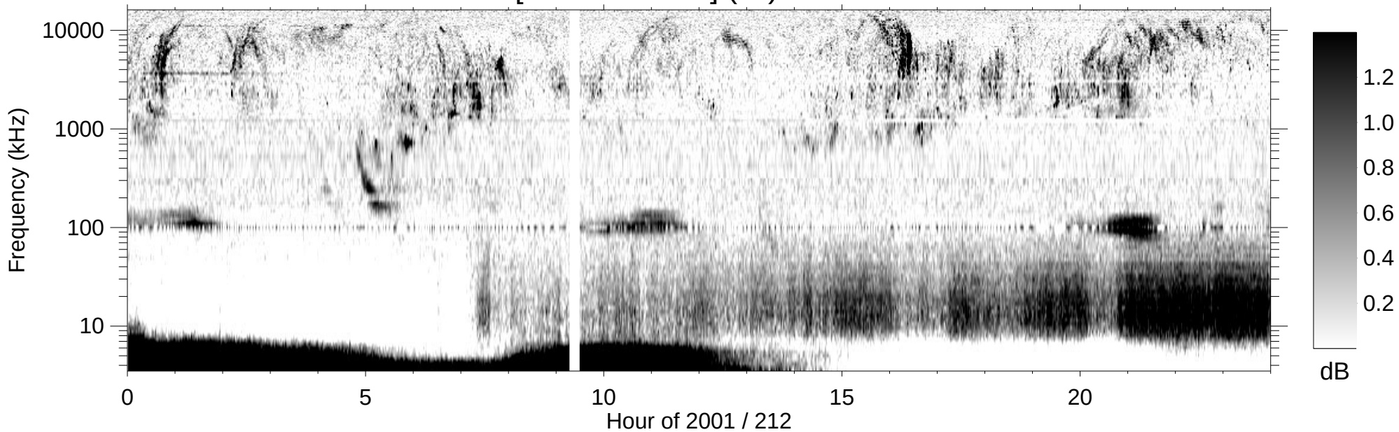
RPWS [ABCH1H2/Ex] (-B) 2001/07/31
