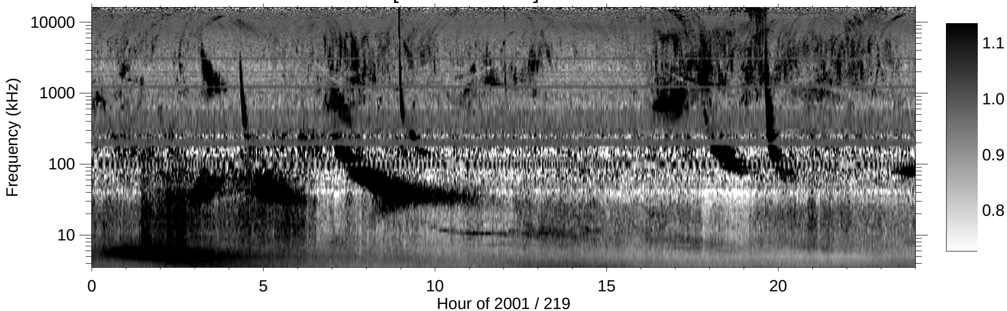
RPWS [ABCH1H2/Ex] (-B) 2001/08/07
