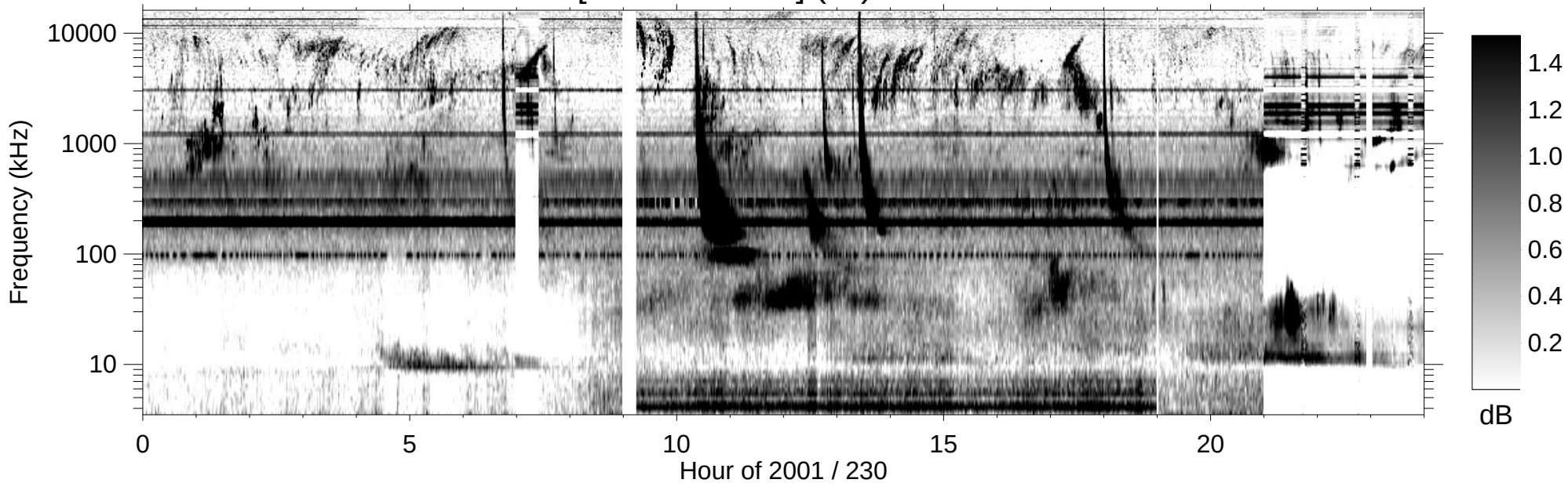
RPWS [ABCH1H2/Ex] (-B) 2001/08/18
