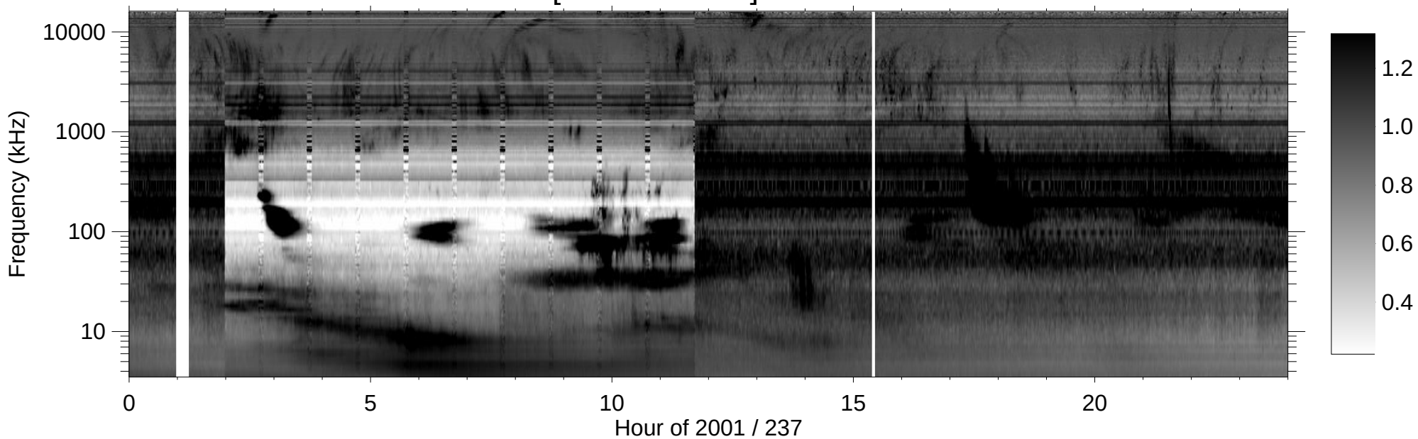
RPWS [ABCH1H2/Ex] (-B) 2001/08/25
