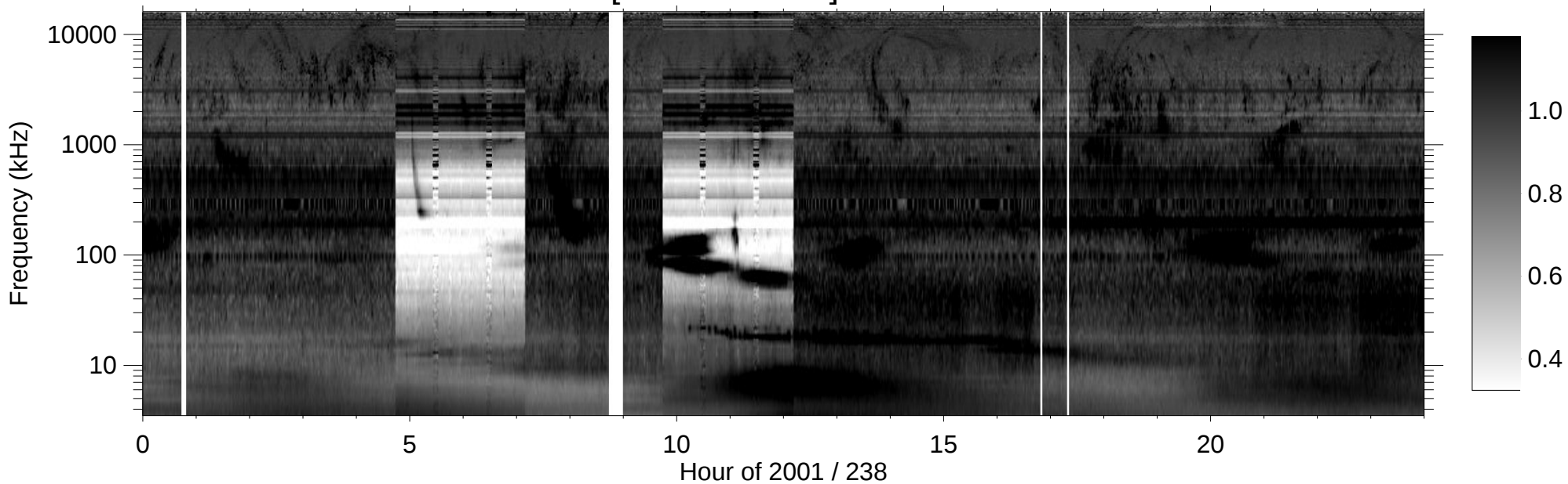
RPWS [ABCH1H2/Ex] (-B) 2001/08/26
