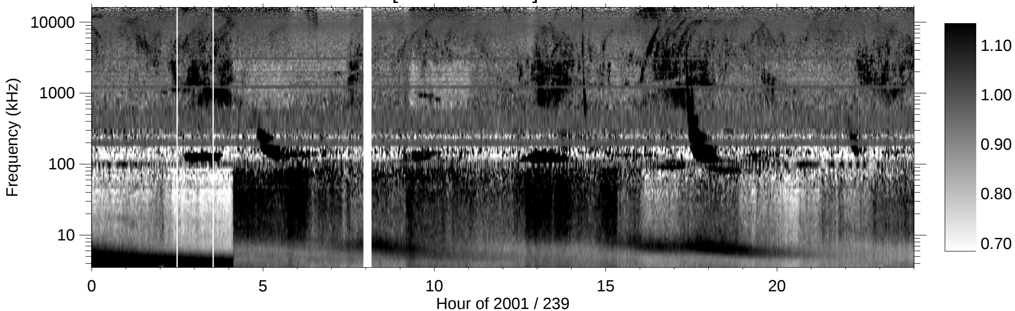
RPWS [ABCH1H2/Ex] (-B) 2001/08/27
