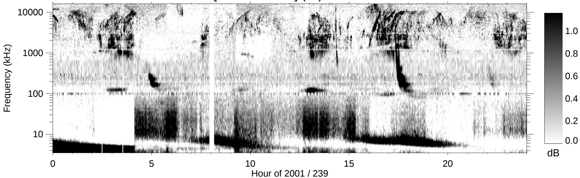
RPWS [ABCH1H2/Ex] (-B) 2001/08/27
