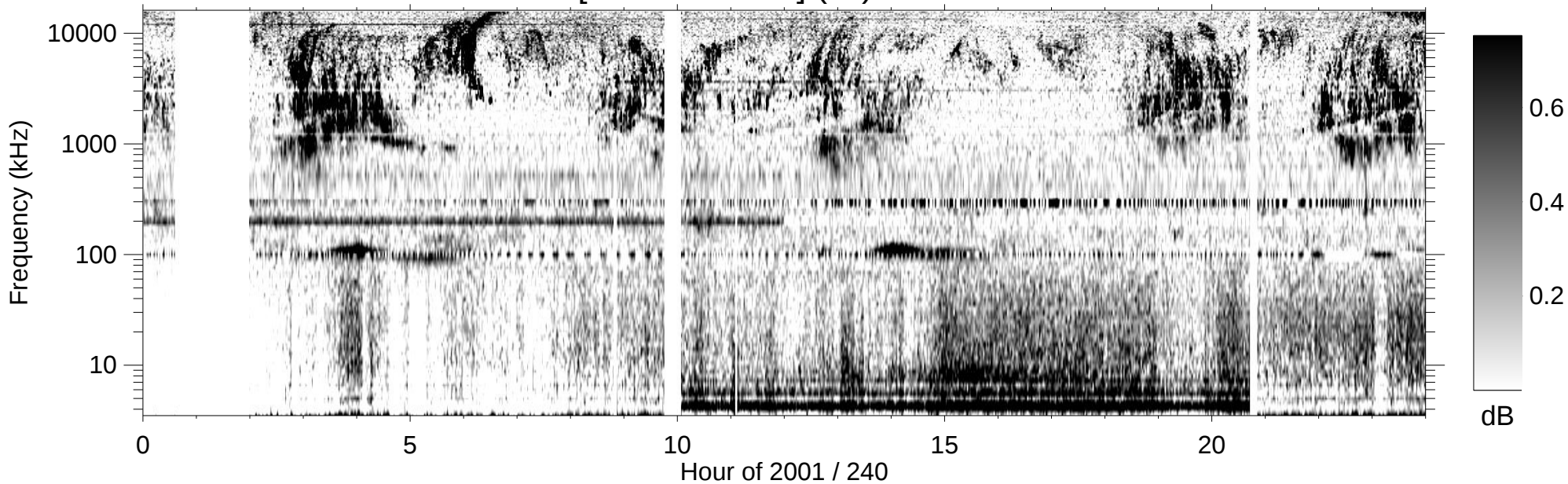
RPWS [ABCH1H2/Ex] (-B) 2001/08/28
