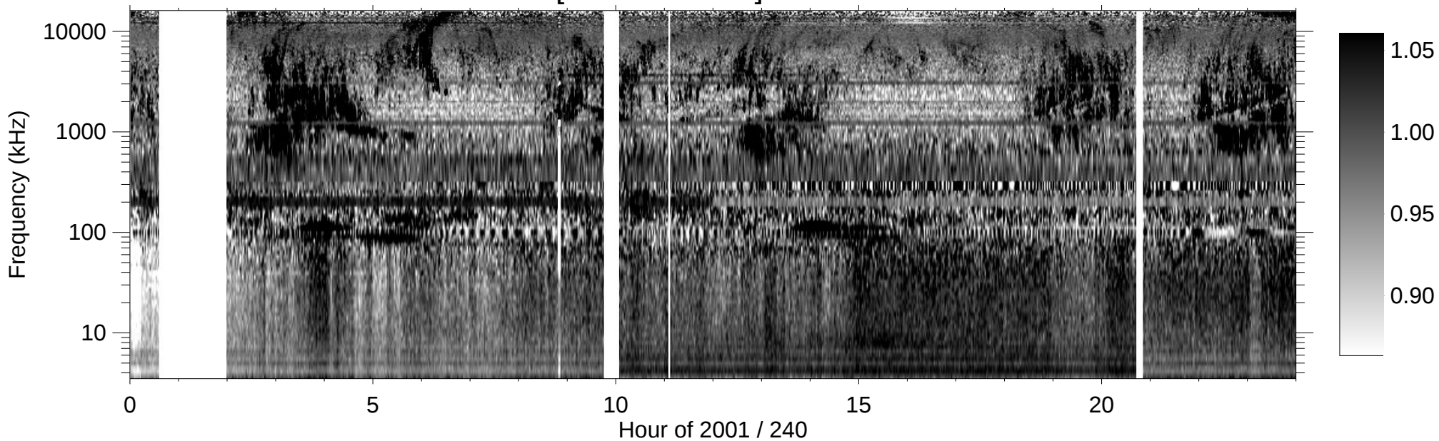
RPWS [ABCH1H2/Ex] (-B) 2001/08/28
