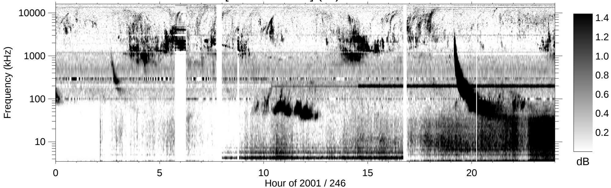
RPWS [ABCH1H2/Ex] (-B) 2001/09/03
