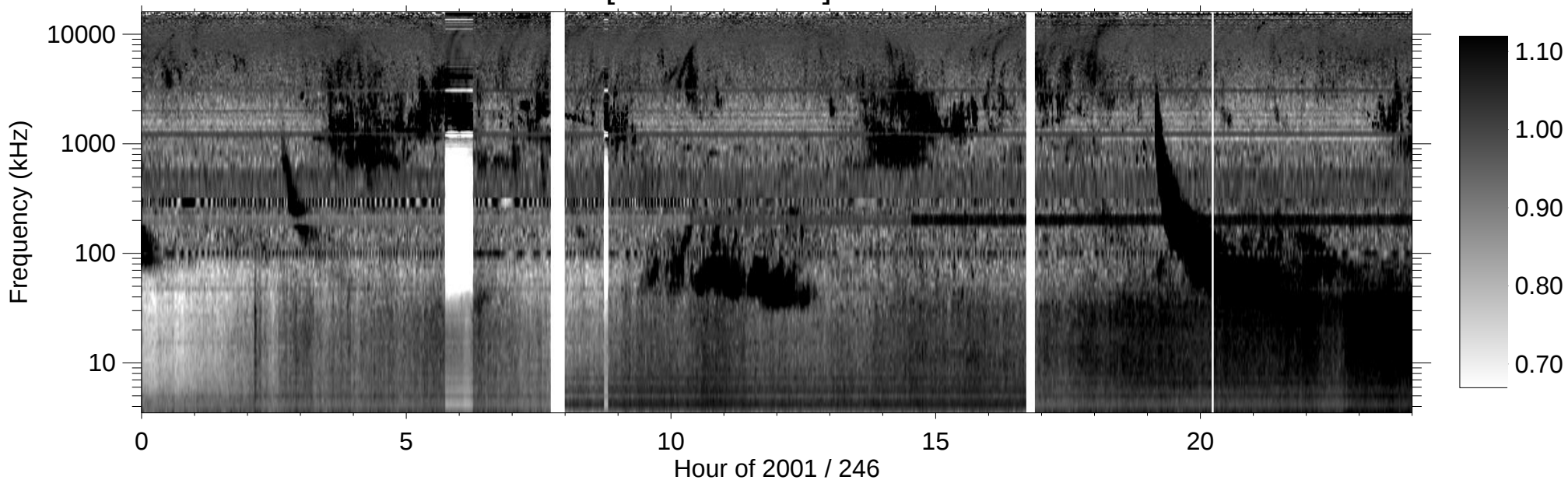
RPWS [ABCH1H2/Ex] (-B) 2001/09/03
