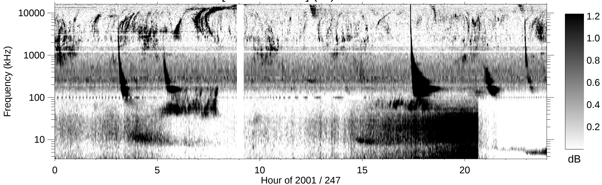
RPWS [ABCH1H2/Ex] (-B) 2001/09/04
