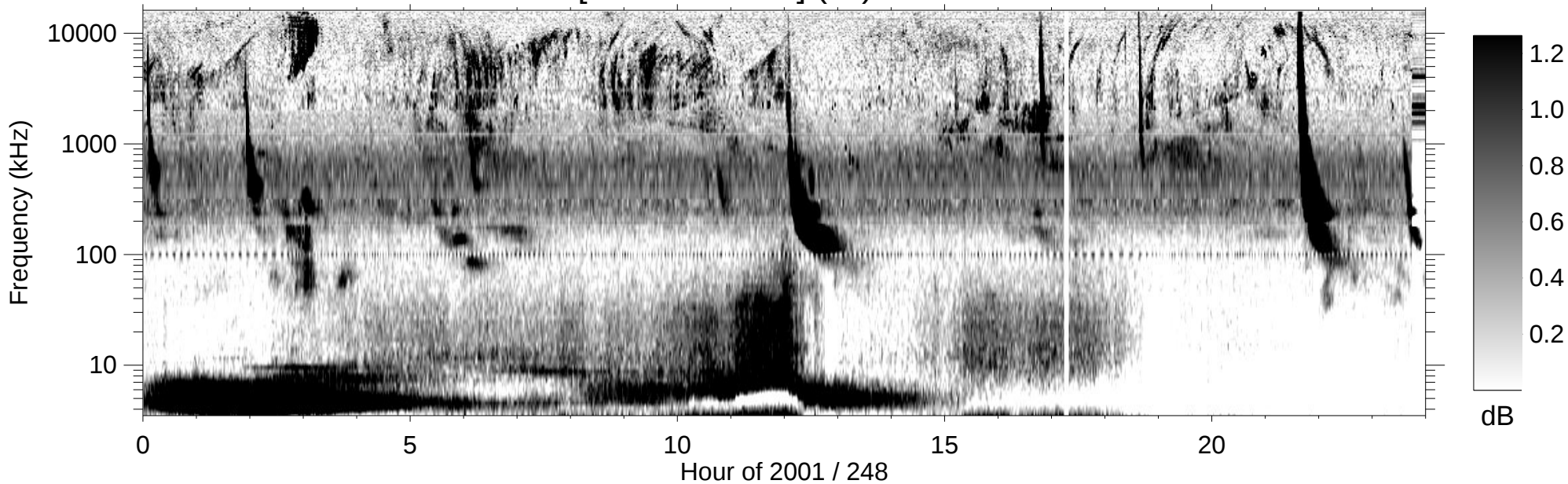
RPWS [ABCH1H2/Ex] (-B) 2001/09/05
