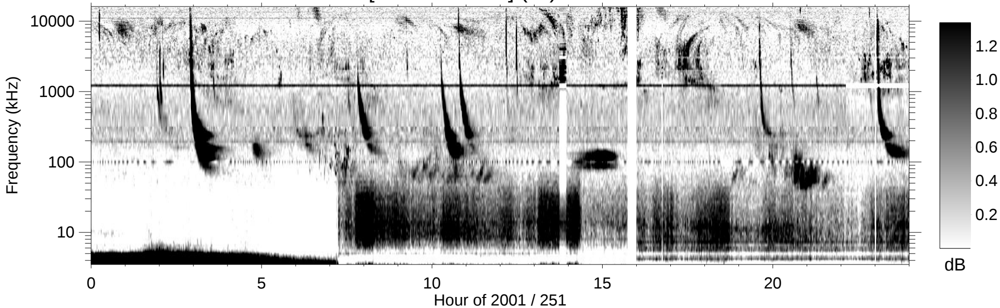
RPWS [ABCH1H2/Ex] (-B) 2001/09/08
