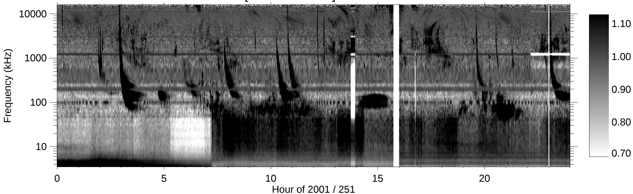
RPWS [ABCH1H2/Ex] (-B) 2001/09/08
