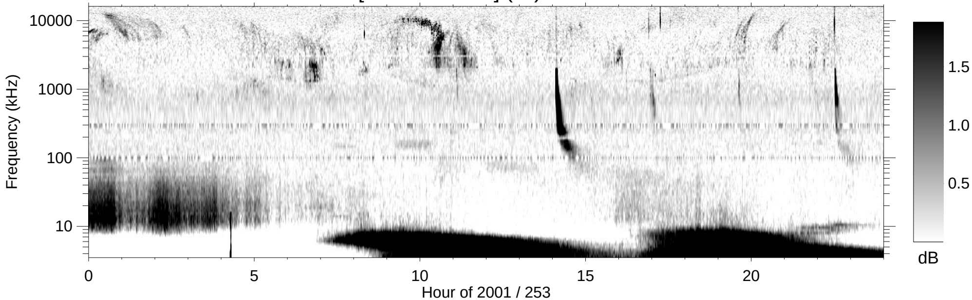
RPWS [ABCH1H2/Ex] (-B) 2001/09/10
