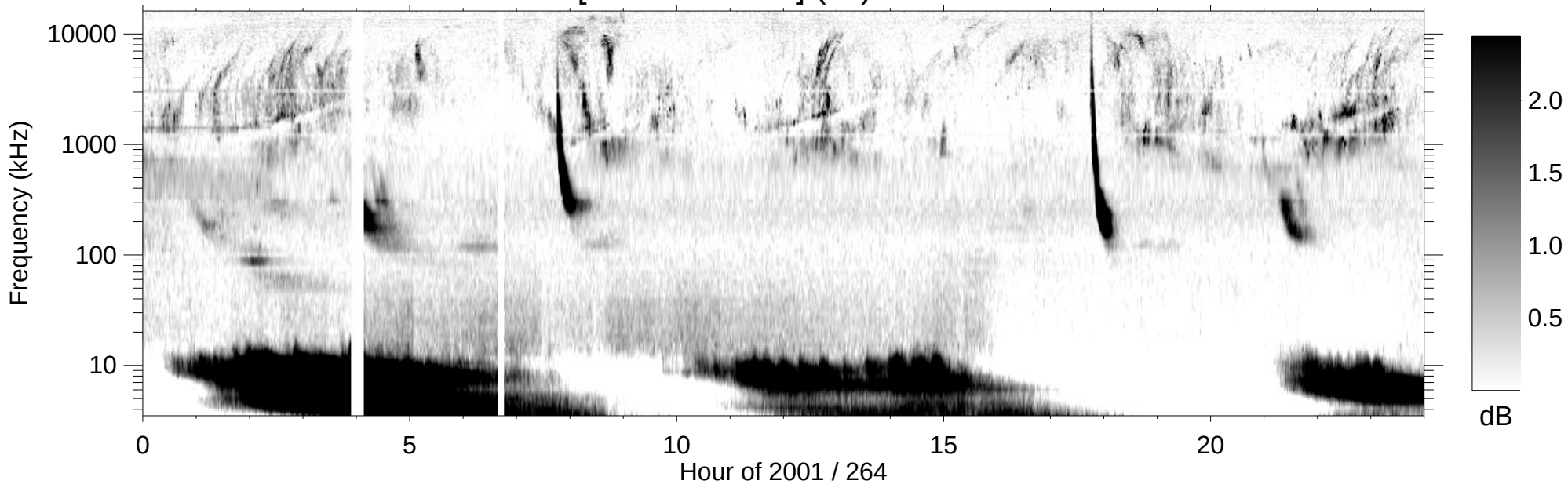
RPWS [ABCH1H2/Ex] (-B) 2001/09/21
