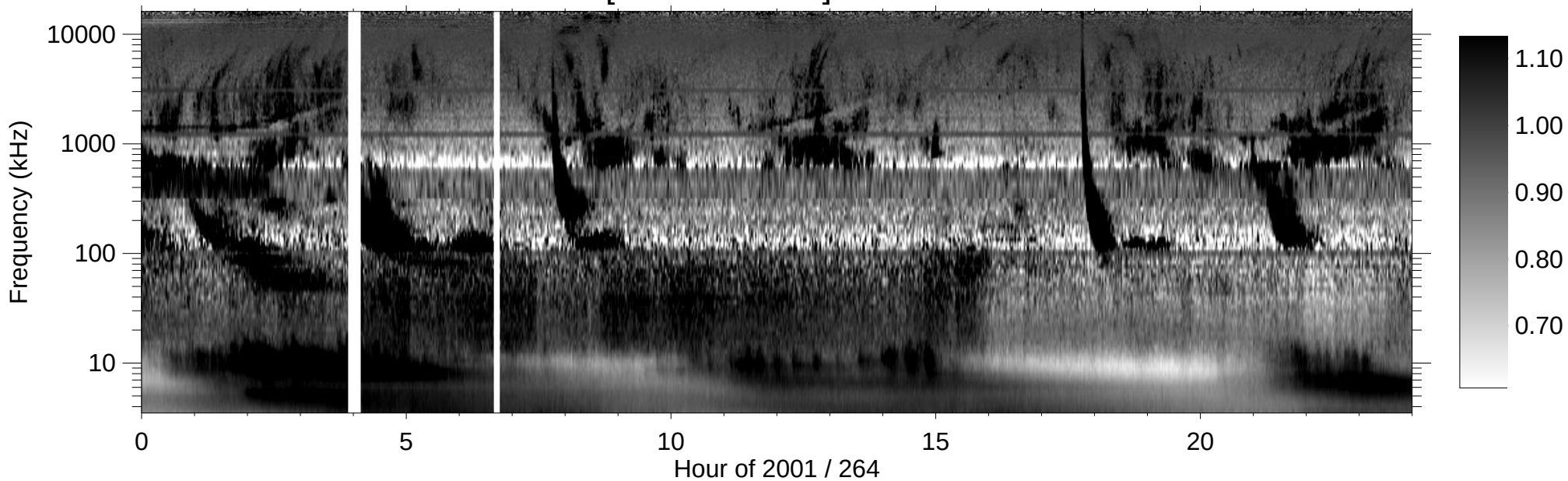
RPWS [ABCH1H2/Ex] (-B) 2001/09/21
