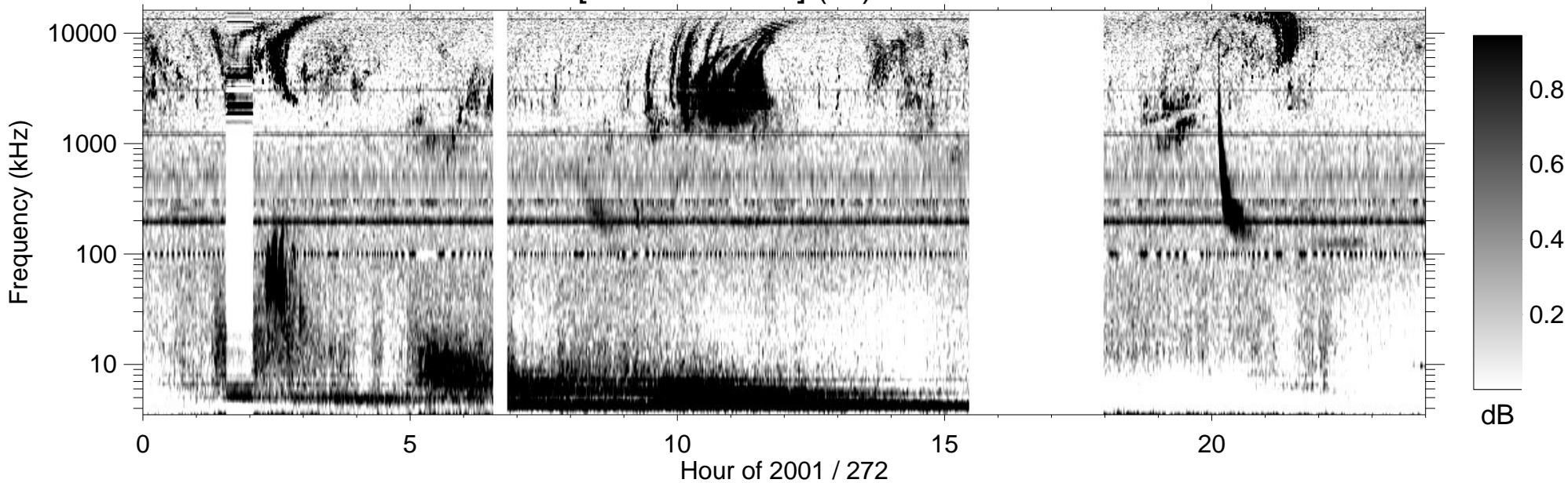
RPWS [ABCH1H2/Ex] (-B) 2001/09/29
