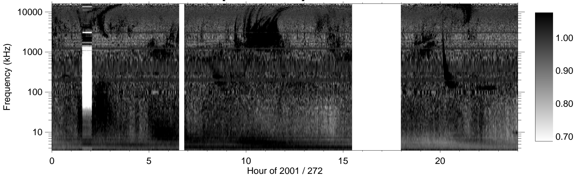
RPWS [ABCH1H2/Ex] (-B) 2001/09/29
