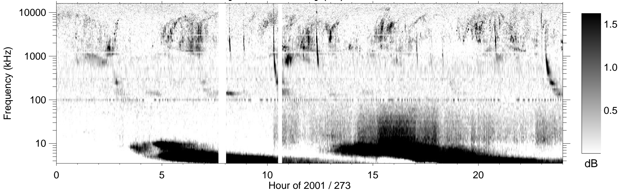
RPWS [ABCH1H2/Ex] (-B) 2001/09/30
