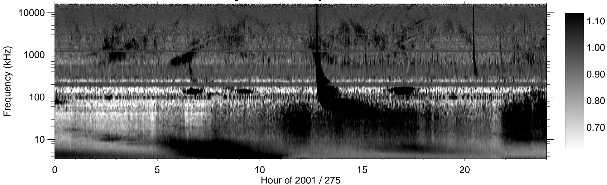
RPWS [ABCH1H2/Ex] (-B) 2001/10/02
