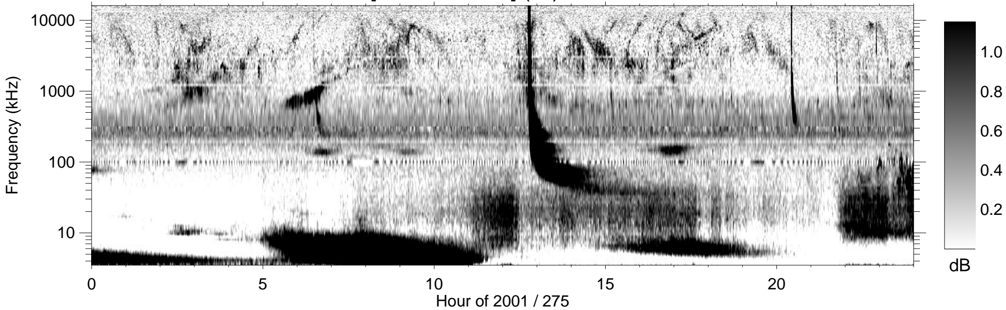
RPWS [ABCH1H2/Ex] (-B) 2001/10/02
