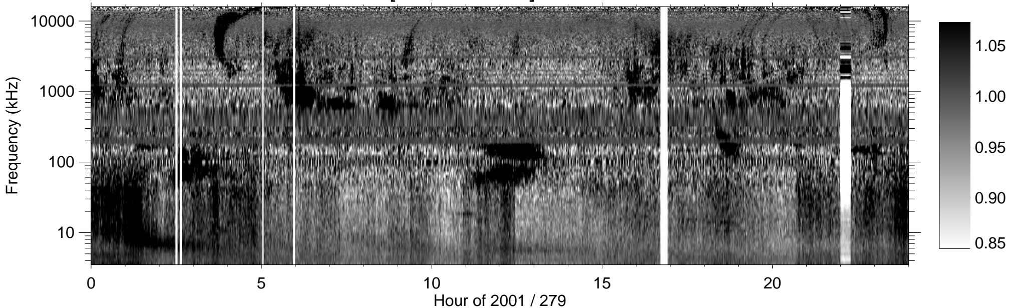
RPWS [ABCH1H2/Ex] (-B) 2001/10/06
