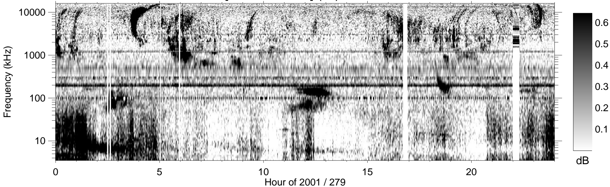
RPWS [ABCH1H2/Ex] (-B) 2001/10/06
