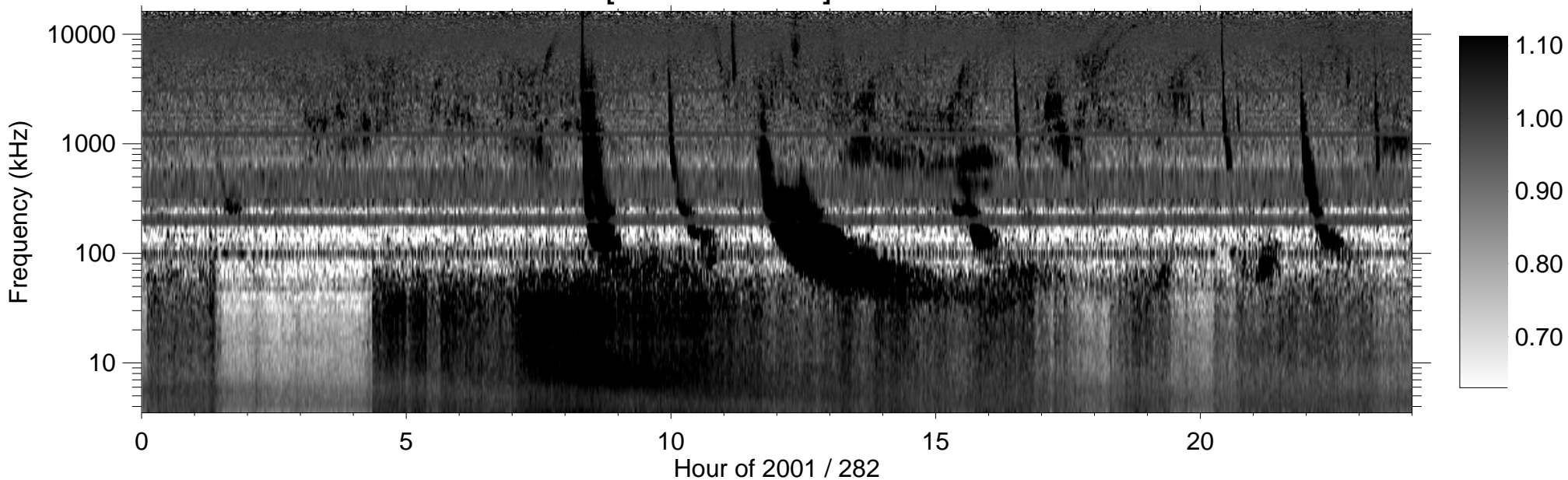
RPWS [ABCH1H2/Ex] (-B) 2001/10/09
