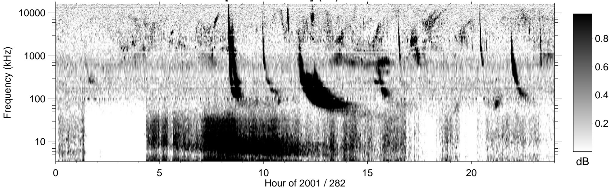
RPWS [ABCH1H2/Ex] (-B) 2001/10/09
