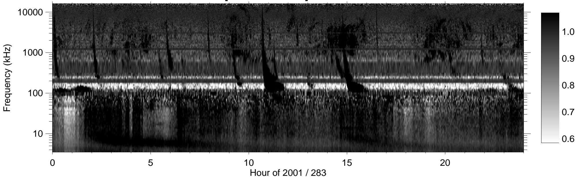
RPWS [ABCH1H2/Ex] (-B) 2001/10/10
