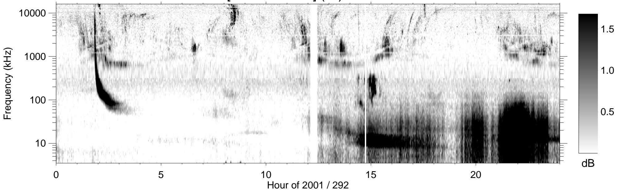
RPWS [ABCH1H2/Ex] (-B) 2001/10/19
