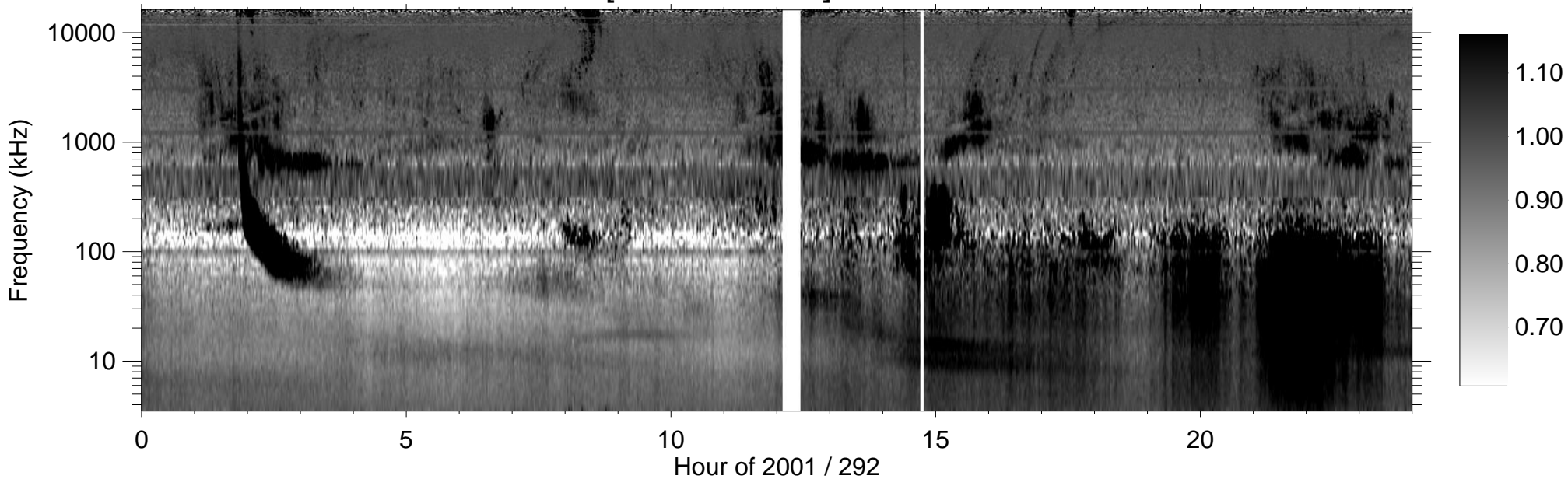
RPWS [ABCH1H2/Ex] (-B) 2001/10/19
