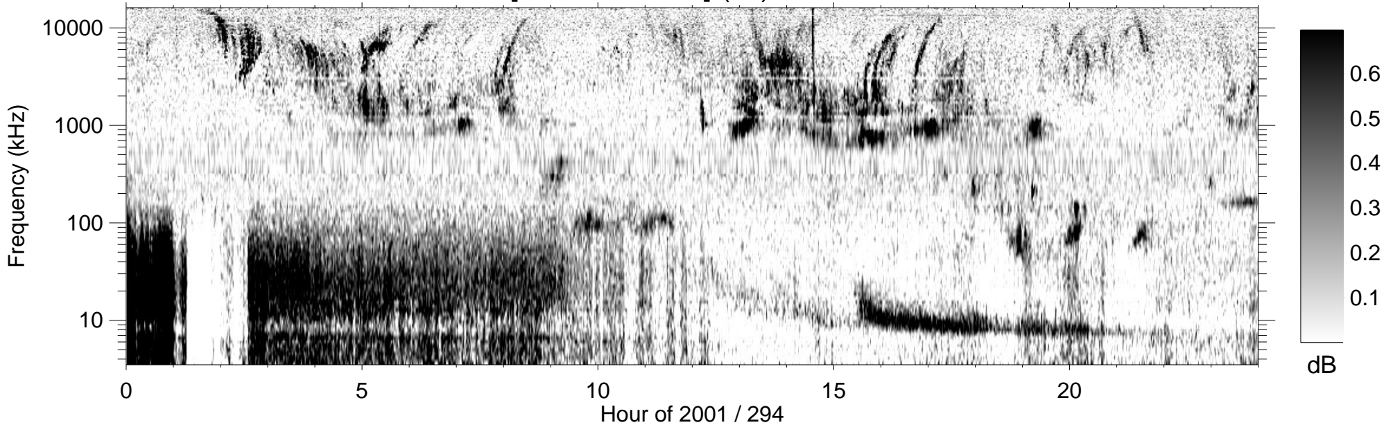
RPWS [ABCH1H2/Ex] (-B) 2001/10/21
