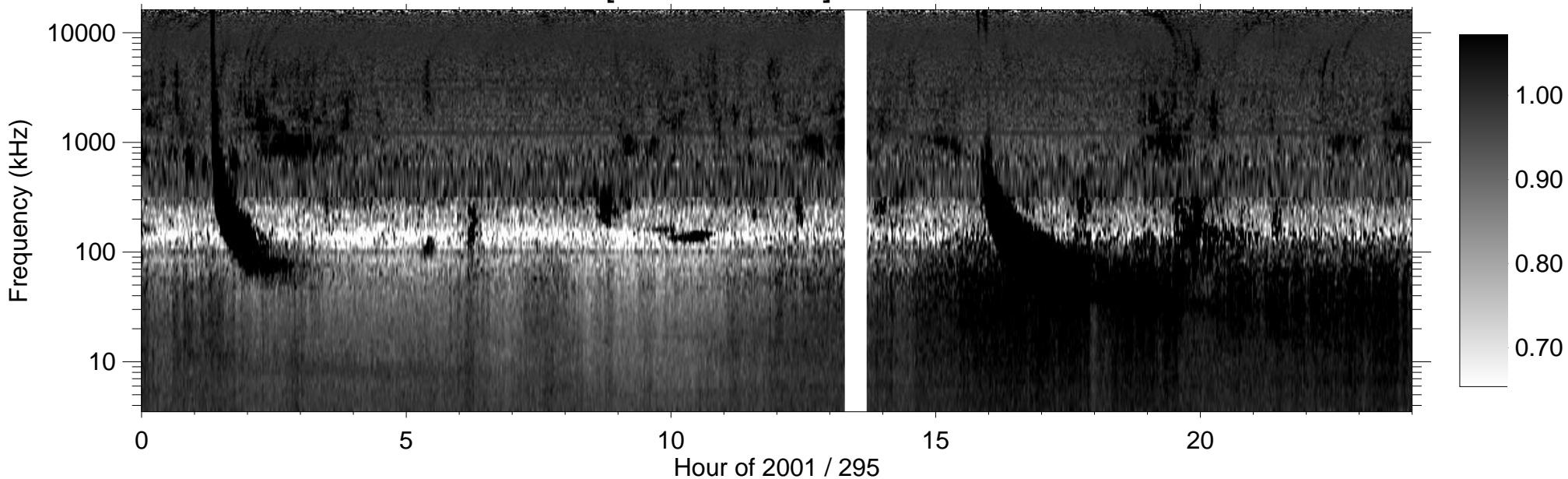
RPWS [ABCH1H2/Ex] (-B) 2001/10/22
