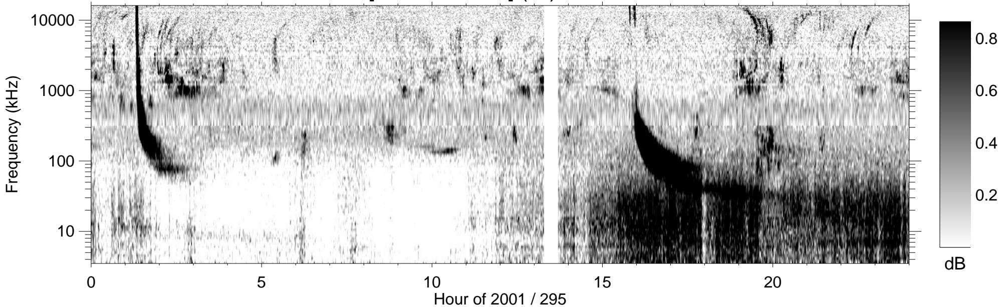
RPWS [ABCH1H2/Ex] (-B) 2001/10/22
