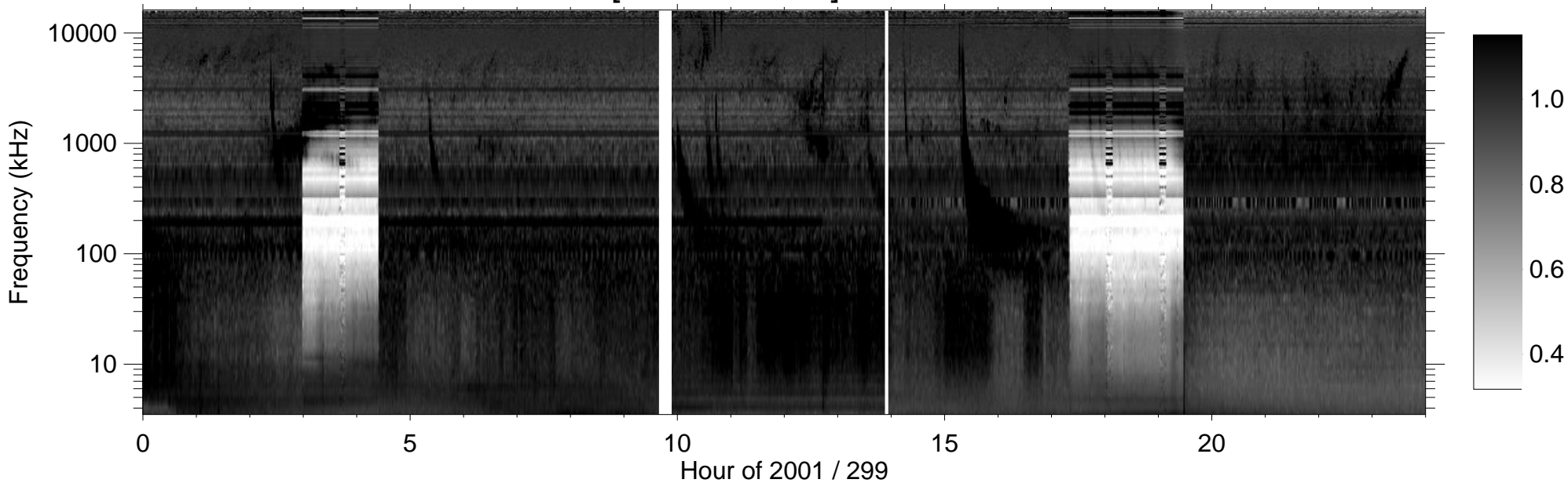
RPWS [ABCH1H2/Ex] (-B) 2001/10/26
