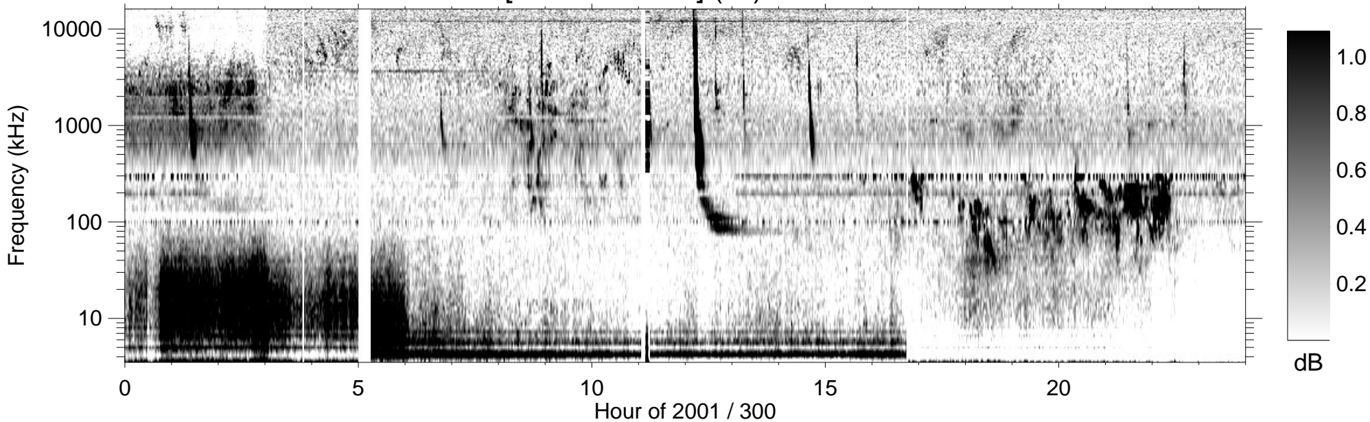
RPWS [ABCH1H2/Ex] (-B) 2001/10/27
