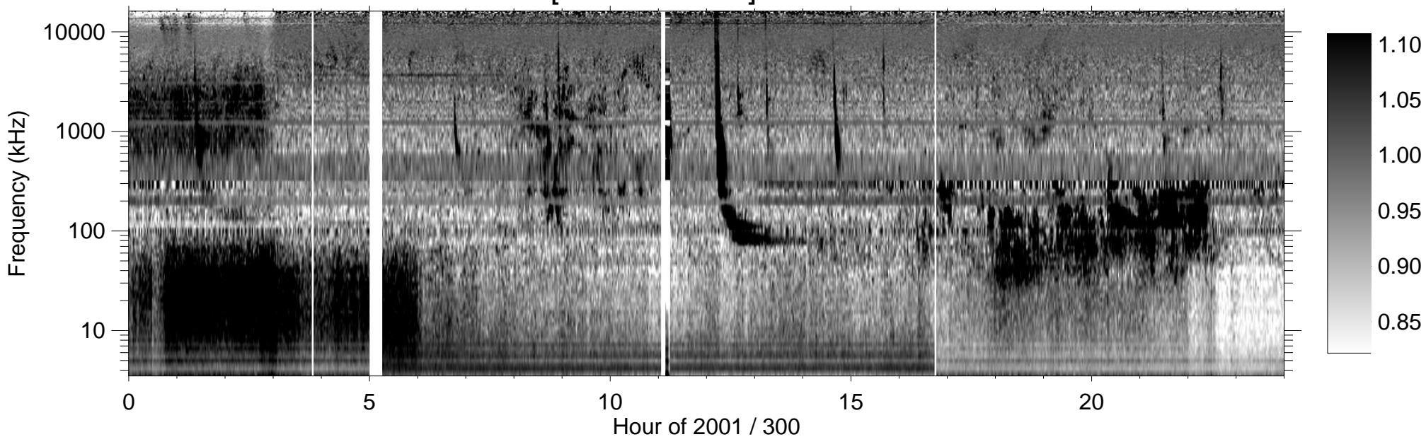
RPWS [ABCH1H2/Ex] (-B) 2001/10/27
