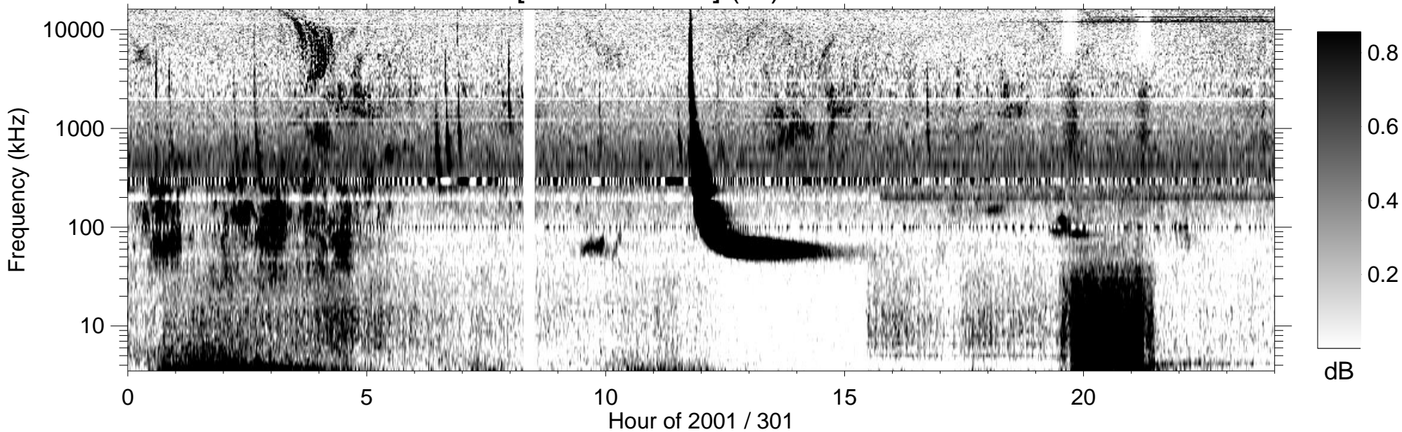
RPWS [ABCH1H2/Ex] (-B) 2001/10/28
