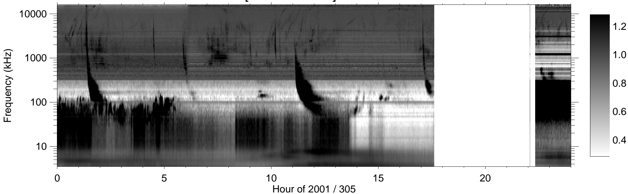
RPWS [ABCH1H2/Ex] (-B) 2001/11/01
