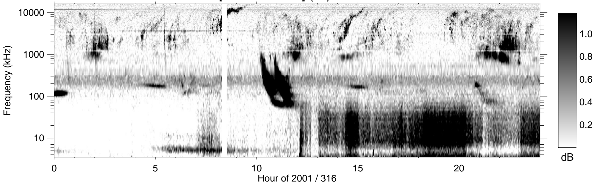
RPWS [ABCH1H2/Ex] (-B) 2001/11/12
