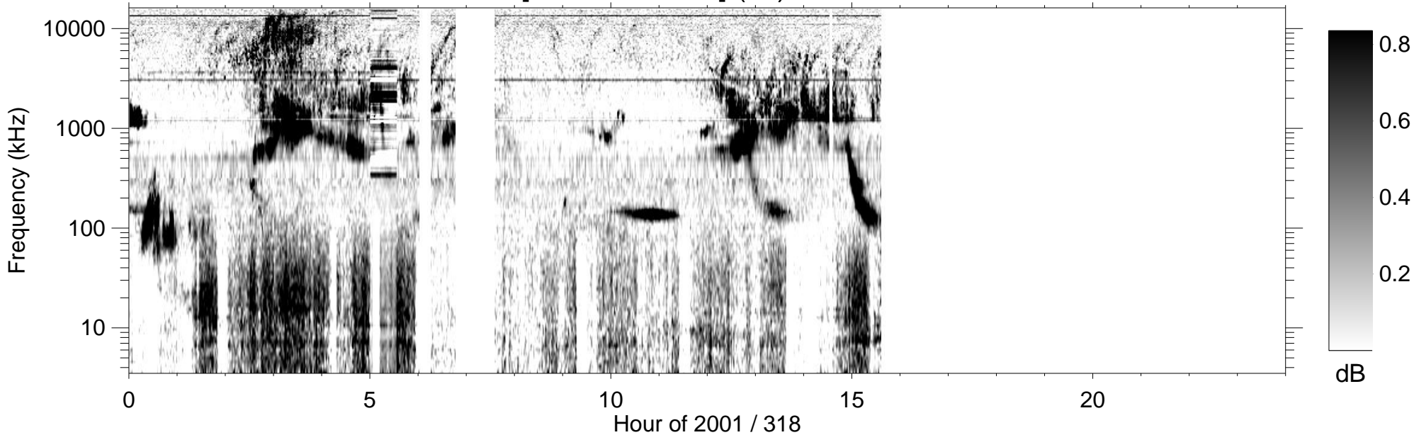
RPWS [ABCH1H2/Ex] (-B) 2001/11/14
