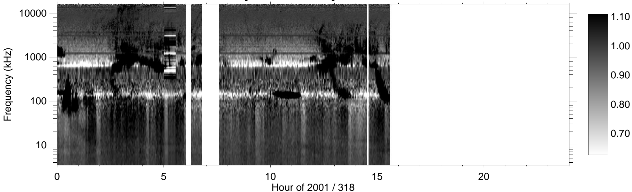
RPWS [ABCH1H2/Ex] (-B) 2001/11/14
