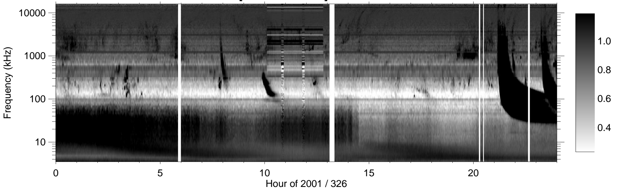
RPWS [ABCH1H2/Ex] (-B) 2001/11/22
