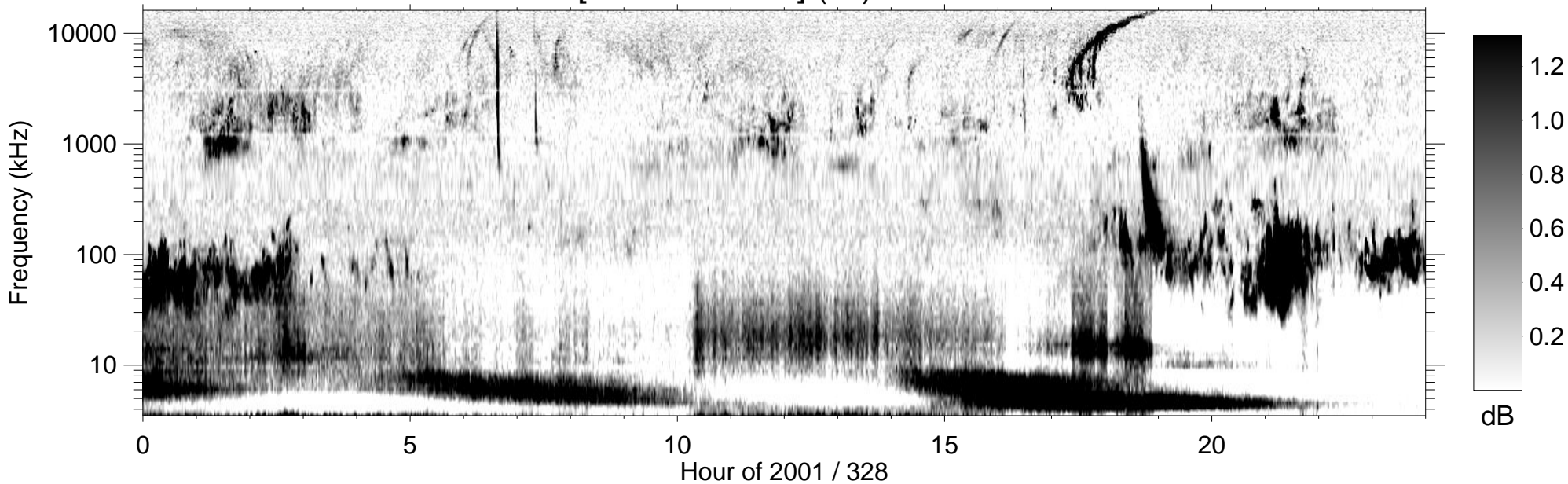
RPWS [ABCH1H2/Ex] (-B) 2001/11/24
