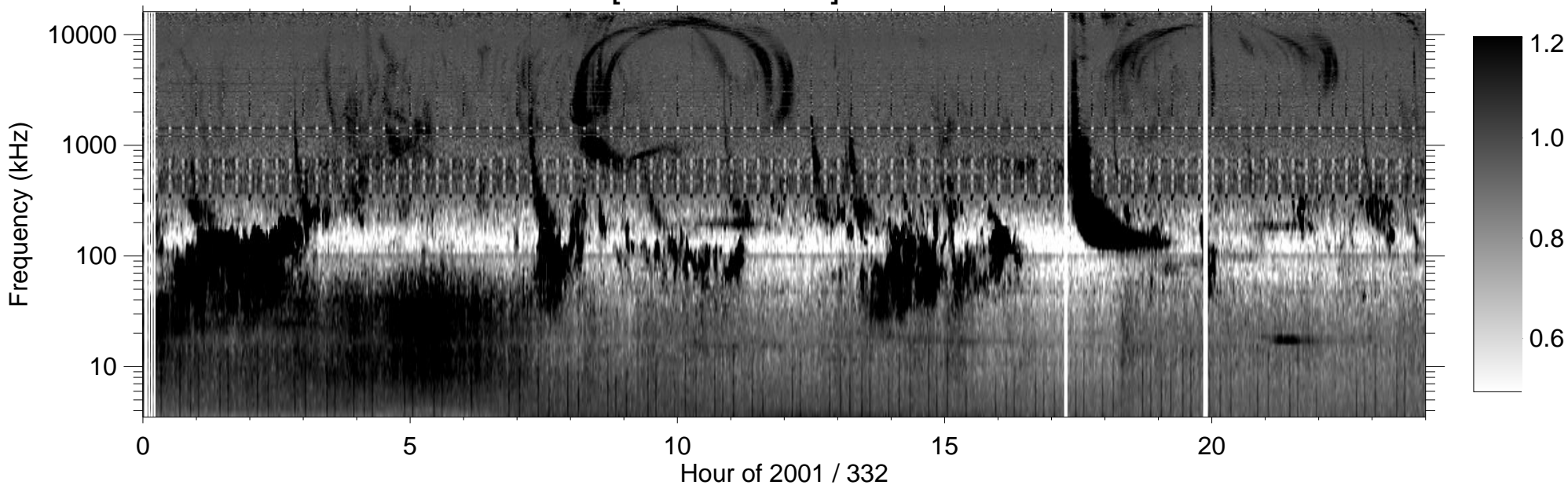
RPWS [ABCH1H2/Ex] (-B) 2001/11/28
