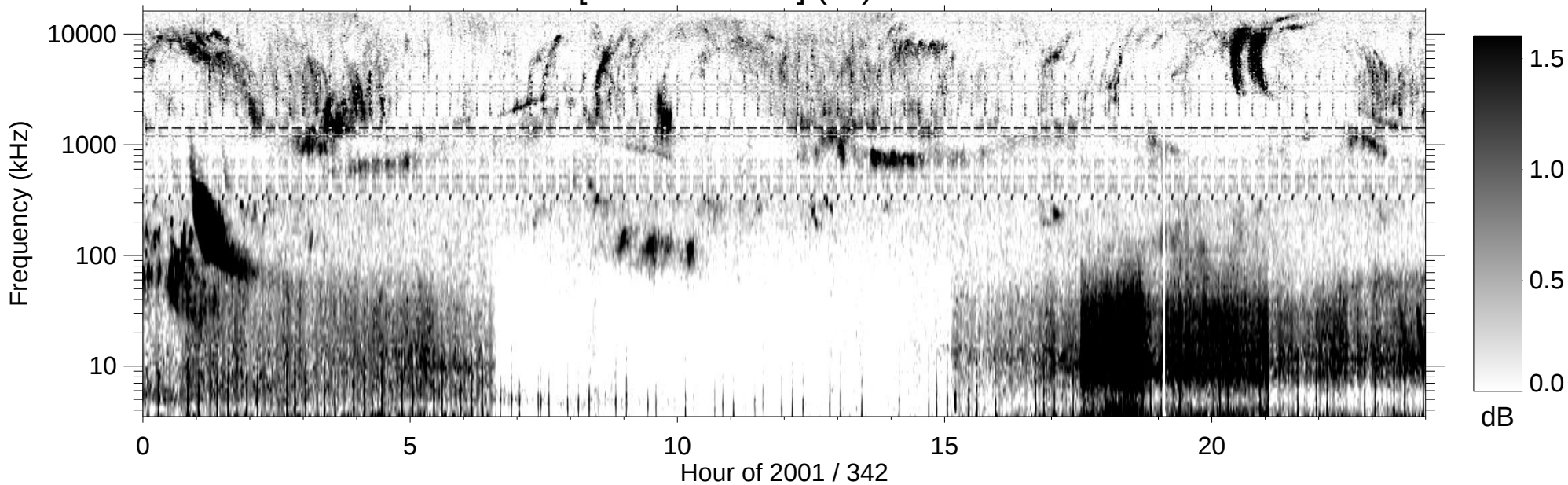
RPWS [ABCH1H2/Ex] (-B) 2001/12/08
