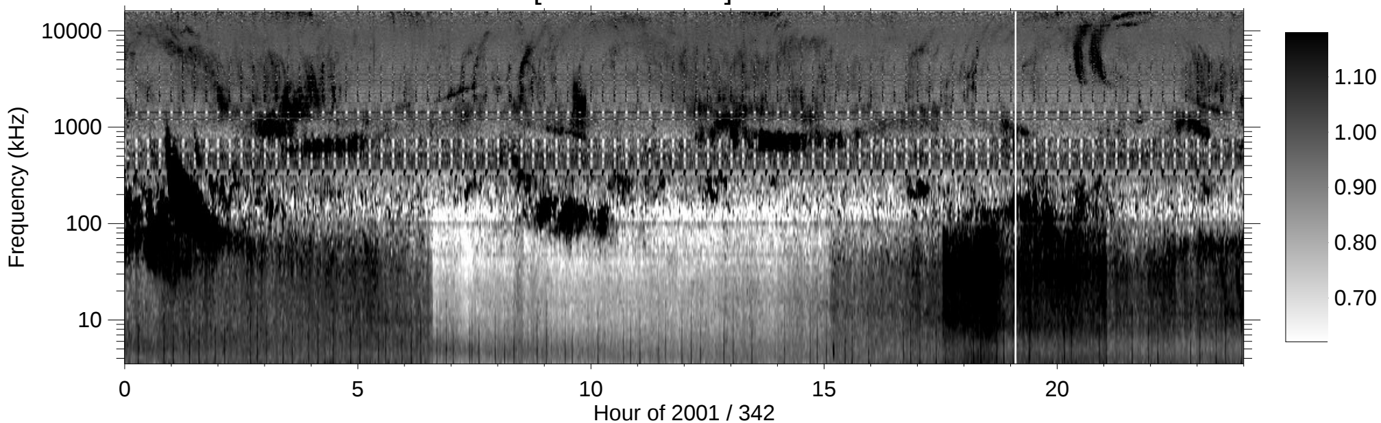
RPWS [ABCH1H2/Ex] (-B) 2001/12/08
