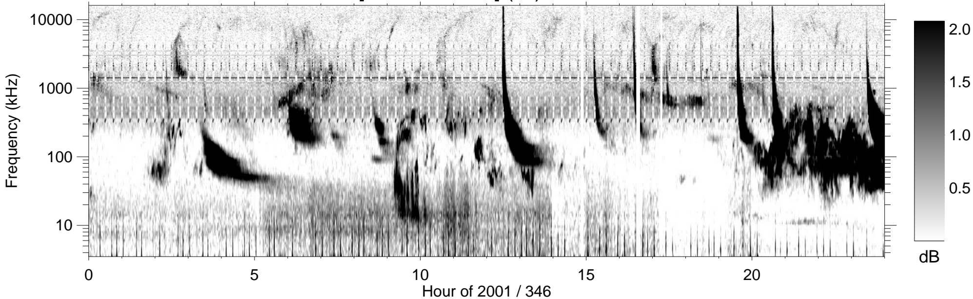
RPWS [ABCH1H2/Ex] (-B) 2001/12/12
