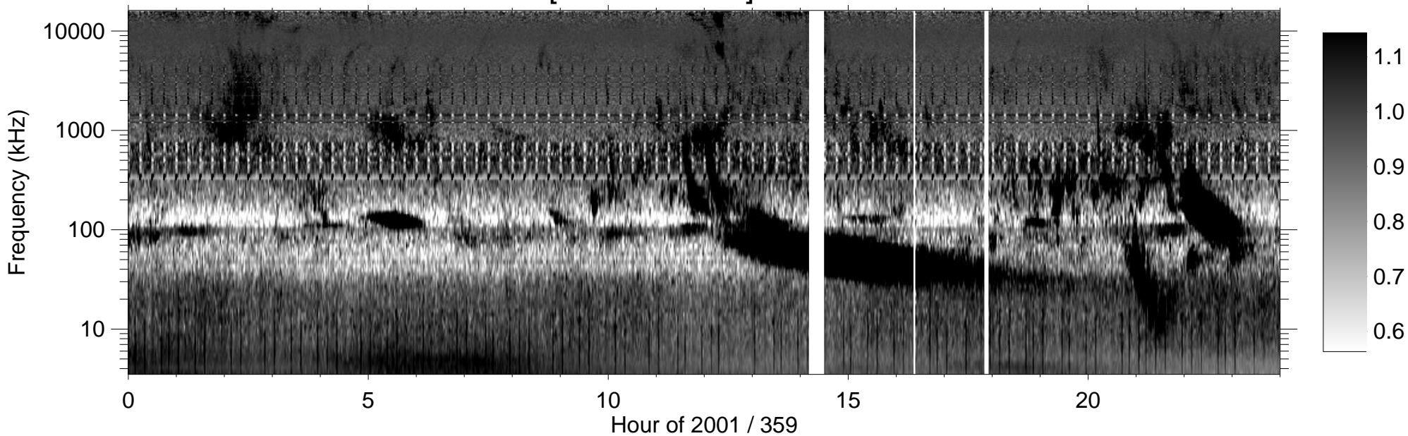
RPWS [ABCH1H2/Ex] (-B) 2001/12/25
