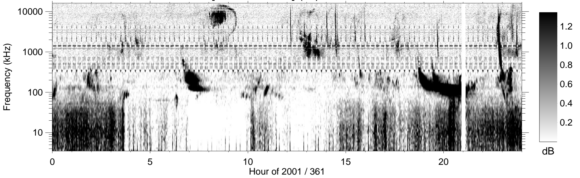
RPWS [ABCH1H2/Ex] (-B) 2001/12/27
