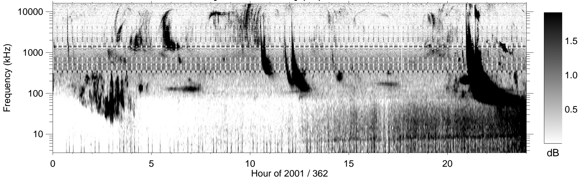
RPWS [ABCH1H2/Ex] (-B) 2001/12/28
