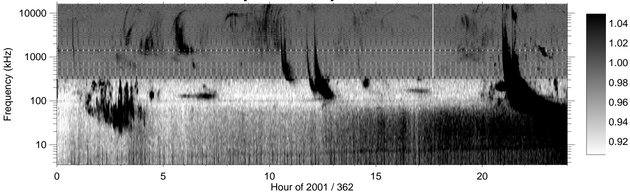
RPWS [ABCH1H2/Ex] (-B) 2001/12/28
