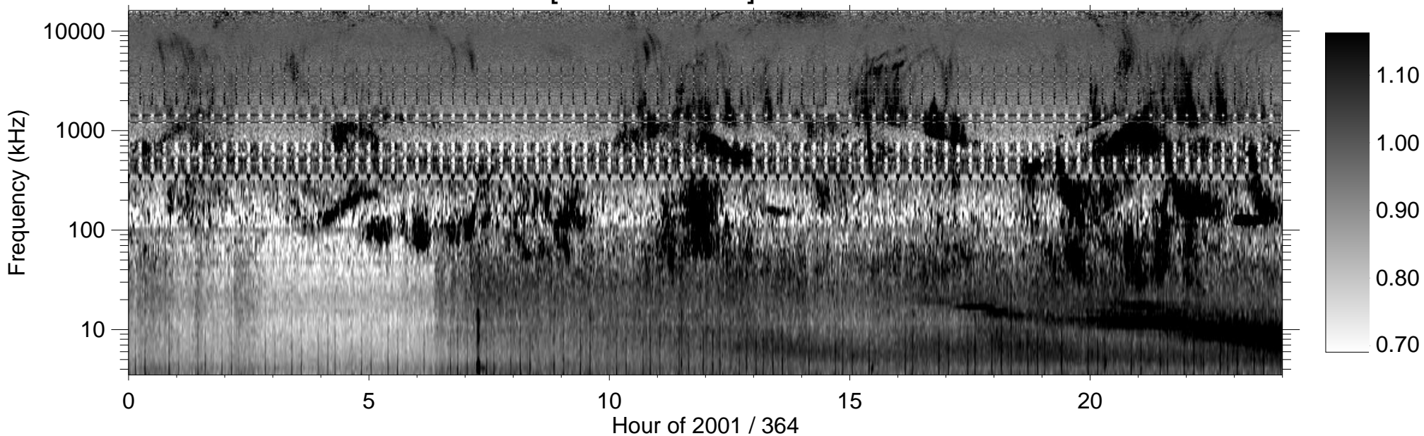
RPWS [ABCH1H2/Ex] (-B) 2001/12/30
