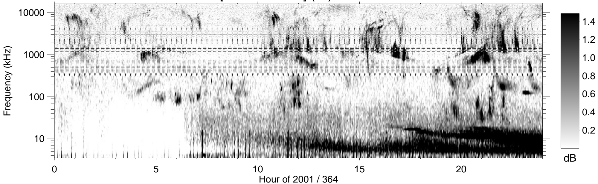
RPWS [ABCH1H2/Ex] (-B) 2001/12/30
