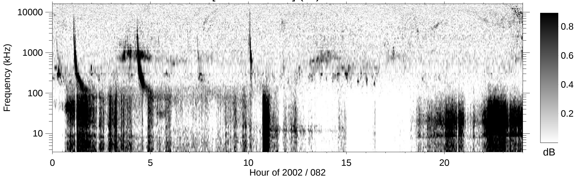
RPWS [ABCH1H2/Ex] (-B) 2002/03/23
