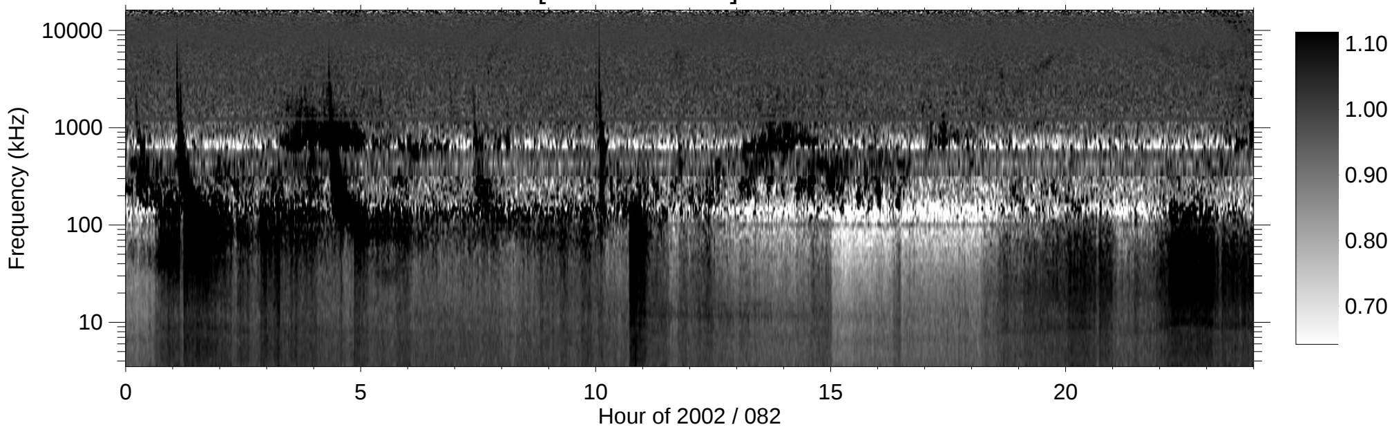
RPWS [ABCH1H2/Ex] (-B) 2002/03/23
