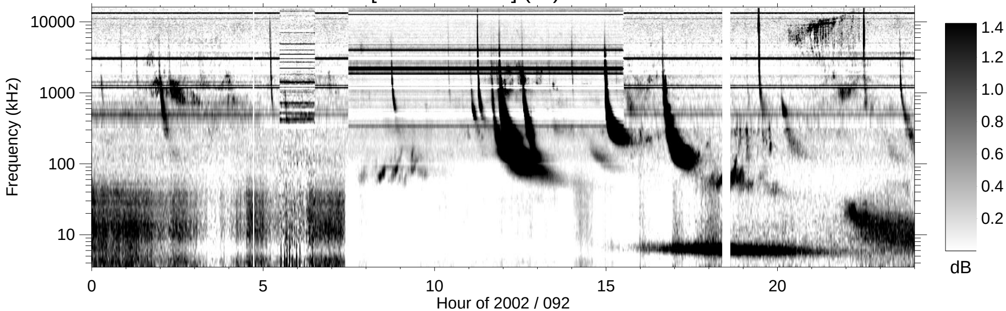
RPWS [ABCH1H2/Ex] (-B) 2002/04/02
