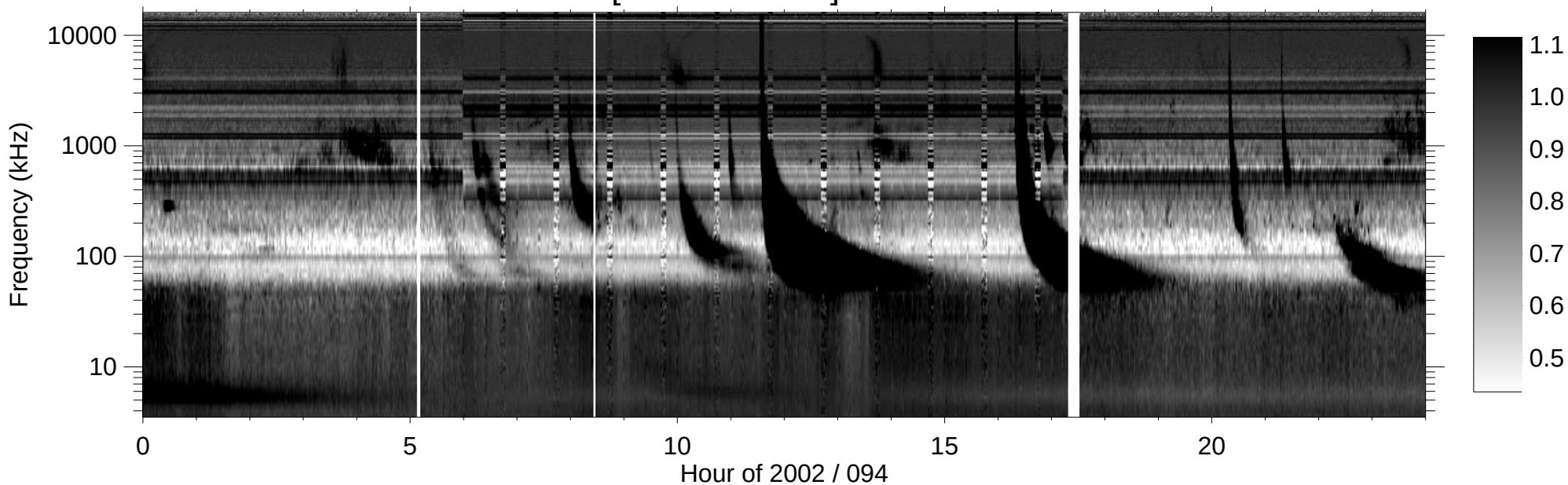
RPWS [ABCH1H2/Ex] (-B) 2002/04/04
