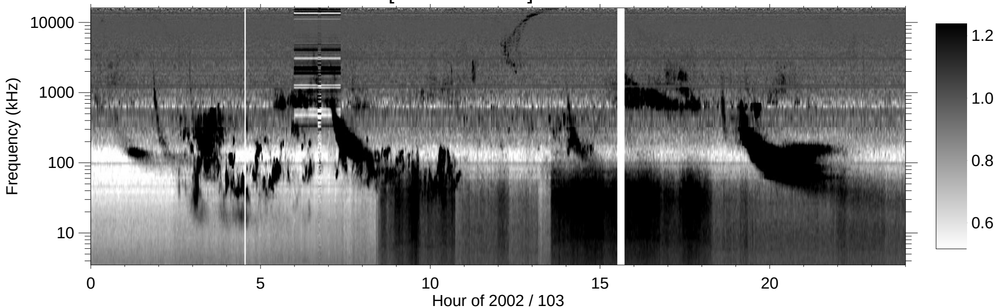
RPWS [ABCH1H2/Ex] (-B) 2002/04/13
