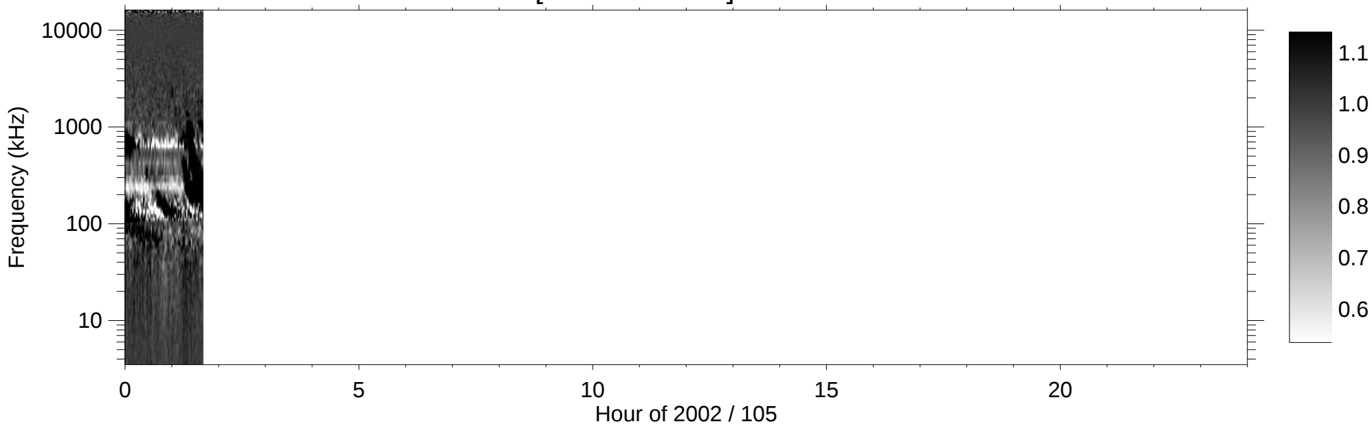
RPWS [ABCH1H2/Ex] (-B) 2002/04/15
