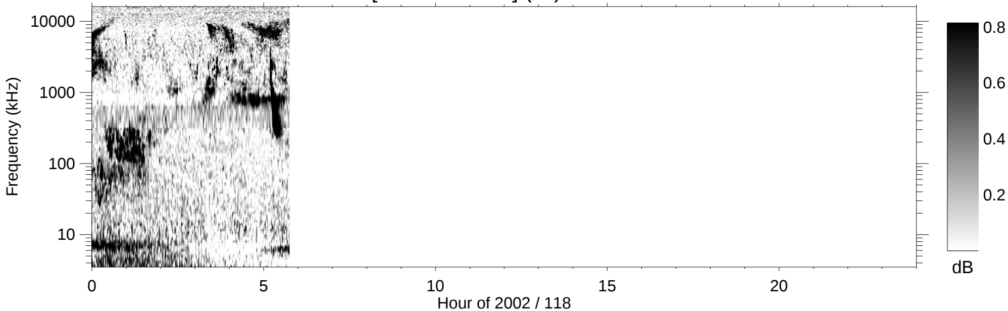
RPWS [ABCH1H2/Ex] (-B) 2002/04/28
