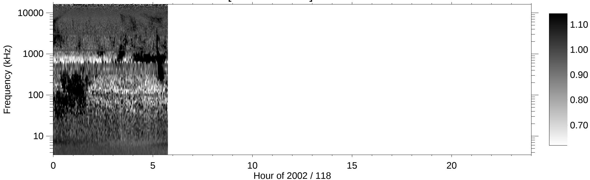
RPWS [ABCH1H2/Ex] (-B) 2002/04/28
